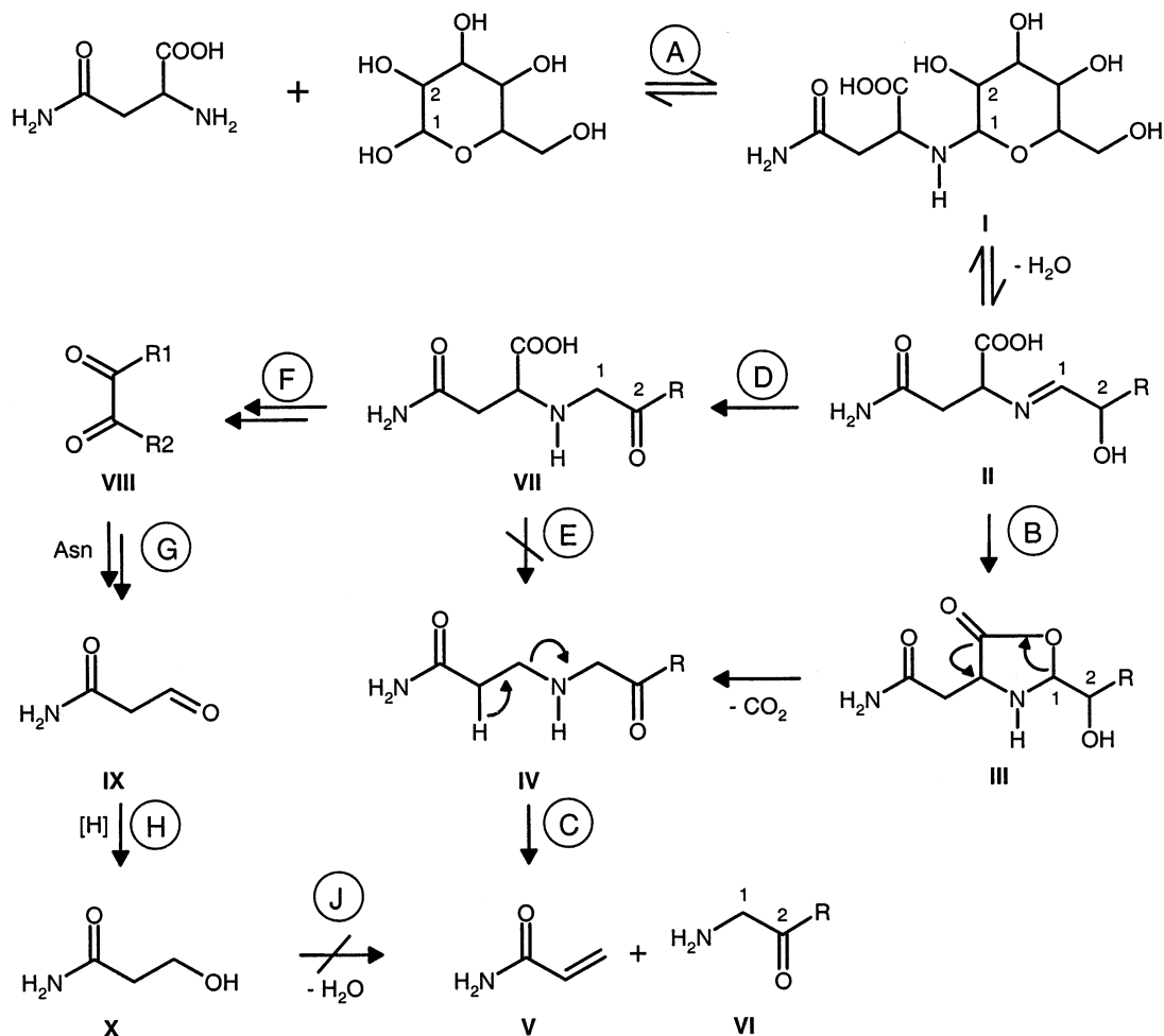
Figure 5 Proposed mechanisms of acrylamide formation in glucose/asparagine coprolylysates through the Maillard reaction.
